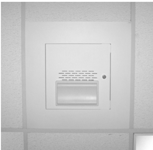
24x24x8 MIMO Ceiling Tile Enclosure – Installed in Ceiling Tile Grid Displayed with a TerraWave 802.11n Dual Band 2.4/5 GHz 2.5/4.5 dBi Ceiling Mount MIMO Omni Antenna and a Cisco 1252 Access Point
