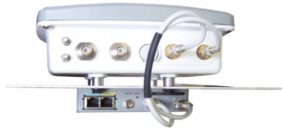
Bottom View of the Cisco 1310 BR, Back Plate and Power Receptacle
