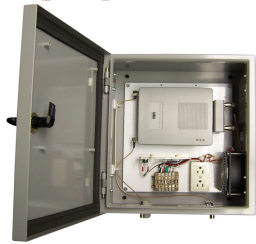
XHC1232 16x12x8 Steel Heated & Cooled Enclosure— Includes the Cisco 1232 Access Point
