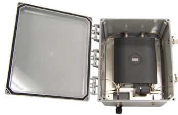
XPS1242-L 12x10x6 Polycarbonate Enclosure with Solid Door and Latch Locks— Includes the Cisco 1242 Access Point
