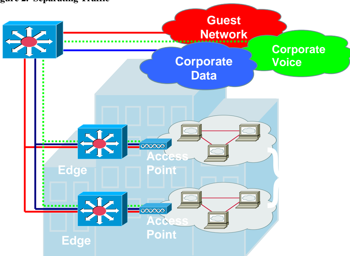
Figure 2. Separating Traffic
