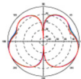
Vertical Radiation Pattern @ 2.4-2.5GHz
