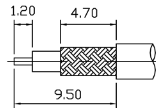
STRIPPING DIMENSION
