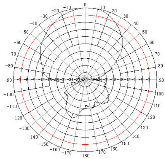
Vertical Radiation Pattern @ 5 GHz
